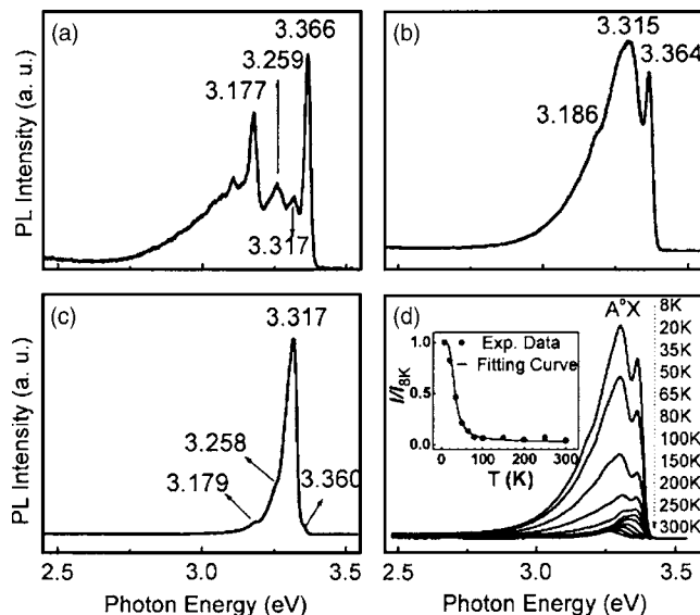
FIG. 4. PL spectra measured at T=8 K for (a) undoped ZnO (sample A), (b) phosphorus-doped ZnO with a GaP cell temperature of 710^\circ\text{C} (sample B), and (c) phosphorus-doped ZnO with a GaP cell temperature of 750^\circ\text{C} (sample C); (d) shows the PL spectra measured for several temperatures over the range from 8 to 300 K (sample B). The inset is the integrated intensity of the A^\circ X emission as a function of temperature. The dots represent the experimental data, and the solid line is the fit.
